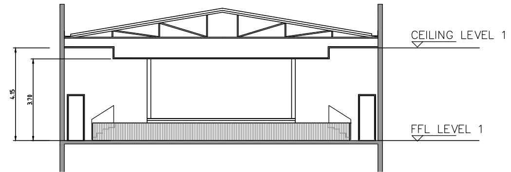
SECTION B
