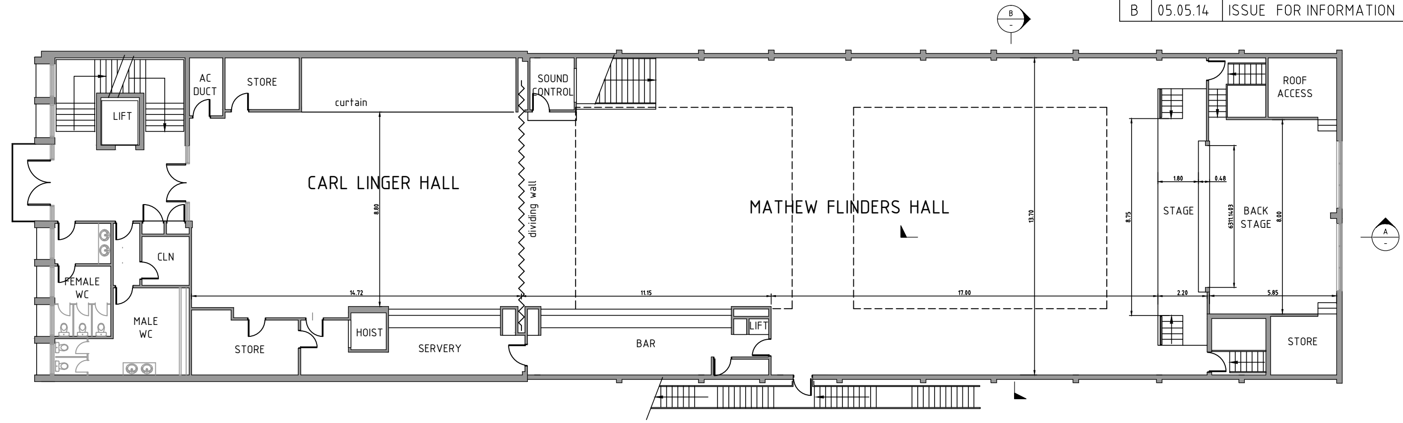
LEVEL 1 FLOOR PLAN
