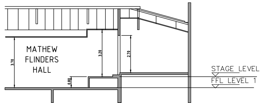
SECTION A
