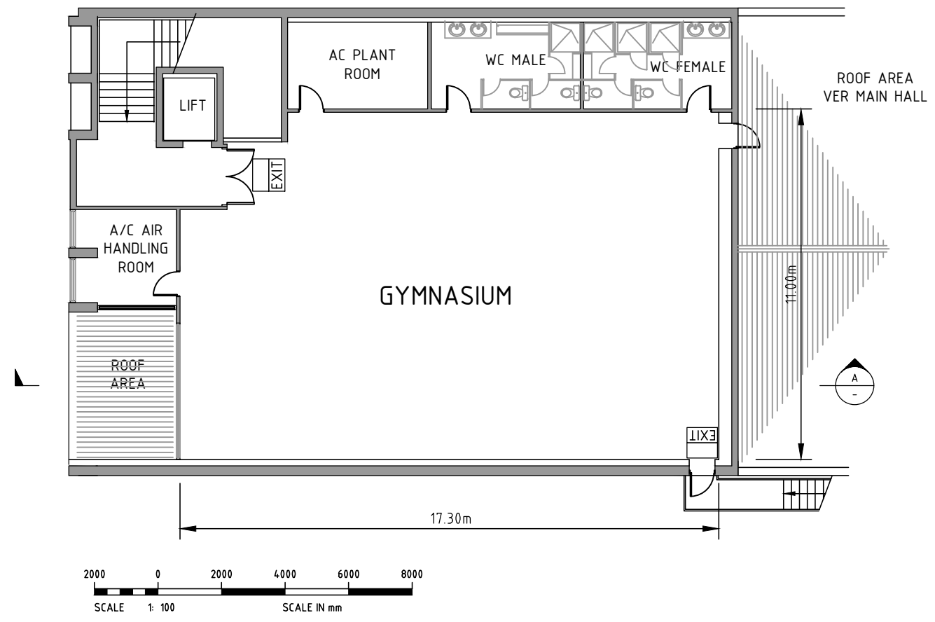
LEVEL 2 FLOOR PLAN
